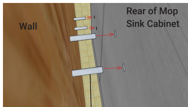
1/2" NPT Piping
